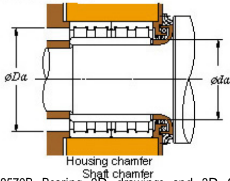
106FC78570B Bearing 2D drawings and 3D CAD models
